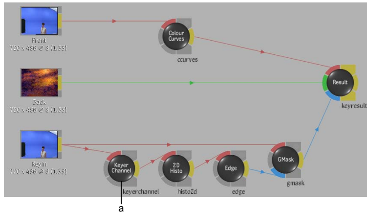
(a) Keyer-Channel node used to pull the key in default processing pipeline Image courtesy of Behavior Communications Inc.
