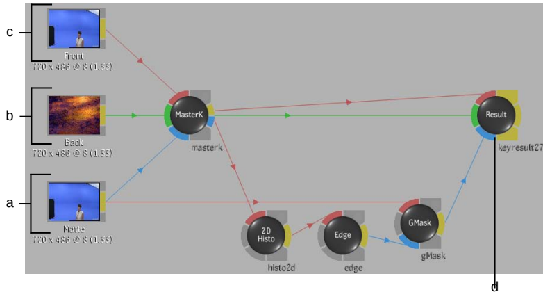
(a) Matte branch (b) Back branch (c) Front branch (d) Result node
