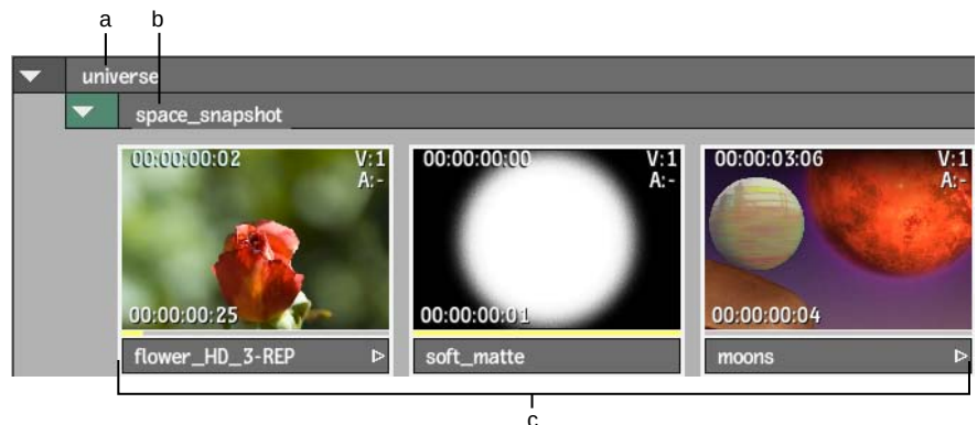
(a) Snapshot library specified in Batch Setup menu (b) Reel entry named according to Batch setup name (c) Source clips saved with Save Setup & Snapshot operation
