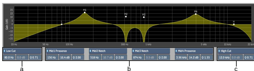
(a) Low Shelf/Cut filter node (b) Mid Notch/Presence filter nodes (c) High Cut/Shelf filter node
