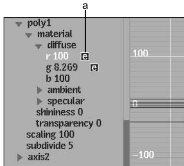
(a) Expression indicator
