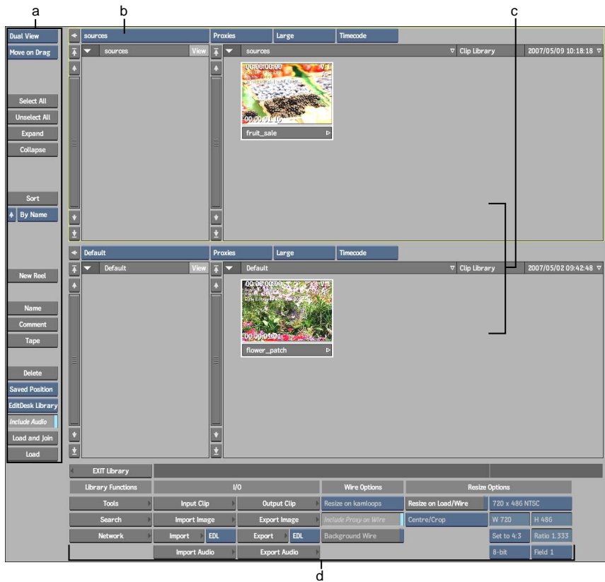
(a) Library Management menu (b) Clip Library box (c) Dual view (d) Clip Library menu
