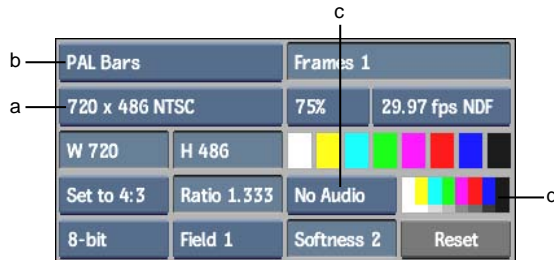
(a) Frame Number field (b) Frame Mode box (c) Current audio tone (d) Current Colour pot
