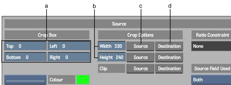
(a) Top, Bottom, Left, Right, Crop fields (b) Crop Box Width/Height fields (c) Source Frame Crop Box button (d) Destination Frame Crop Box button
