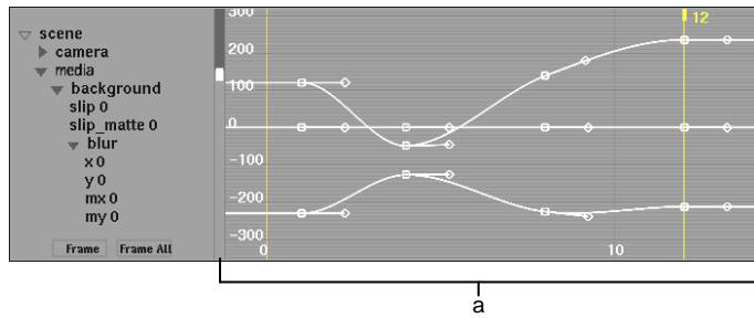
(a) Original animation curve
