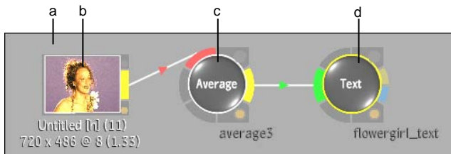
(a) Clip history in Inferno, Flame, and Flint (b) Clip with colour correction, supported in all products (c) Batch module operations supported in Inferno, Flame, and Flint only (d) Text supported in all products
