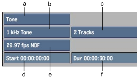
(a) Audio Tools box (b) Frequency box (c) Audio Tracks box (d) Start Time field (e) Timecode mode box (f) Duration field
