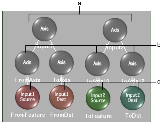
(a) Spline node trees for one Input1, and one Input2 spline (b) Axis nodes for individual spline wireframes (c) Spline nodes for corresponding source and destination splines
