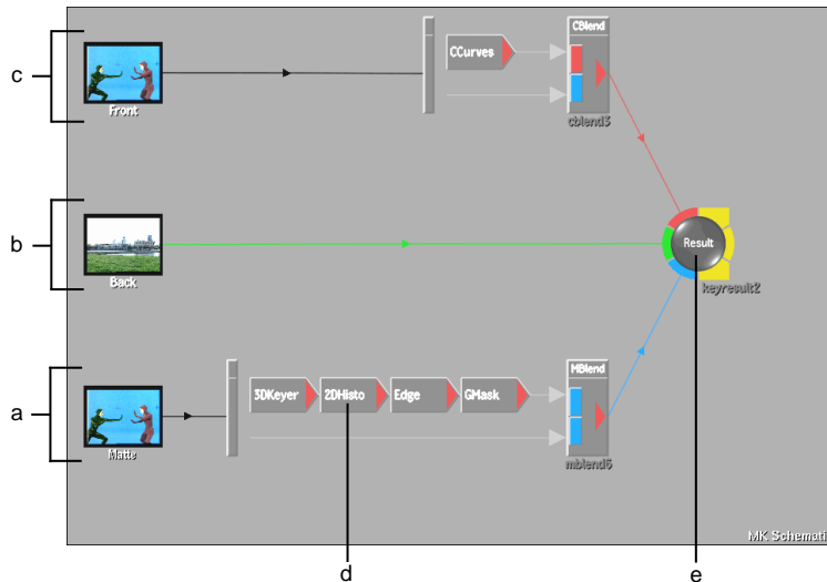
(a) Matte branch (b) Back branch (c) Front branch (d) Process node (e) Result node
