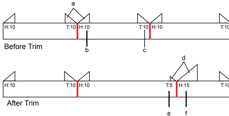
(a) Visual indicator of head/tail size (b) 10 frames are in the head (c) 10 frames are in the tail (d) Visual indicator of the change in head/tail size (e) Result of 5 tail frames trimmed into clip (f) Result of 5 frames trimmed out of clip and into the head
