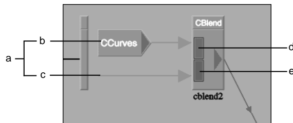
(a) The two pipes constitute one layer (b) Front pipe (c) Matte pipe (d) Red box of Front pipe (e) Blue box of Matte pipe
