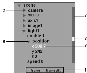
(a) Expanded Position folder (b) Camera folder (c) Scroll bar (d) Indicates the relative position (e) Value (f) Framing buttons
