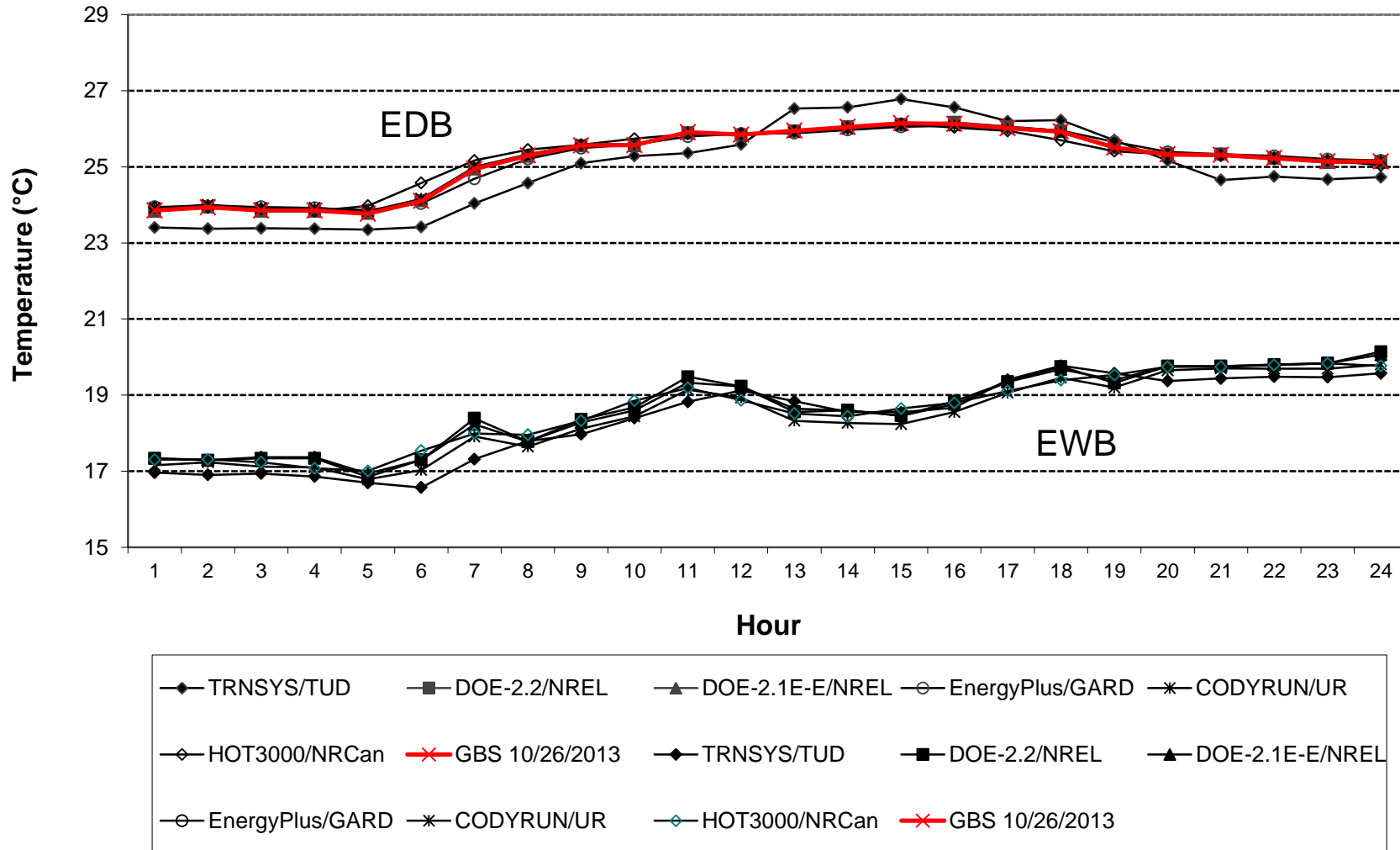
Figure B16.5.2-50. HVAC BESTEST: CE300 June 28 Hourly EDB & EWB
