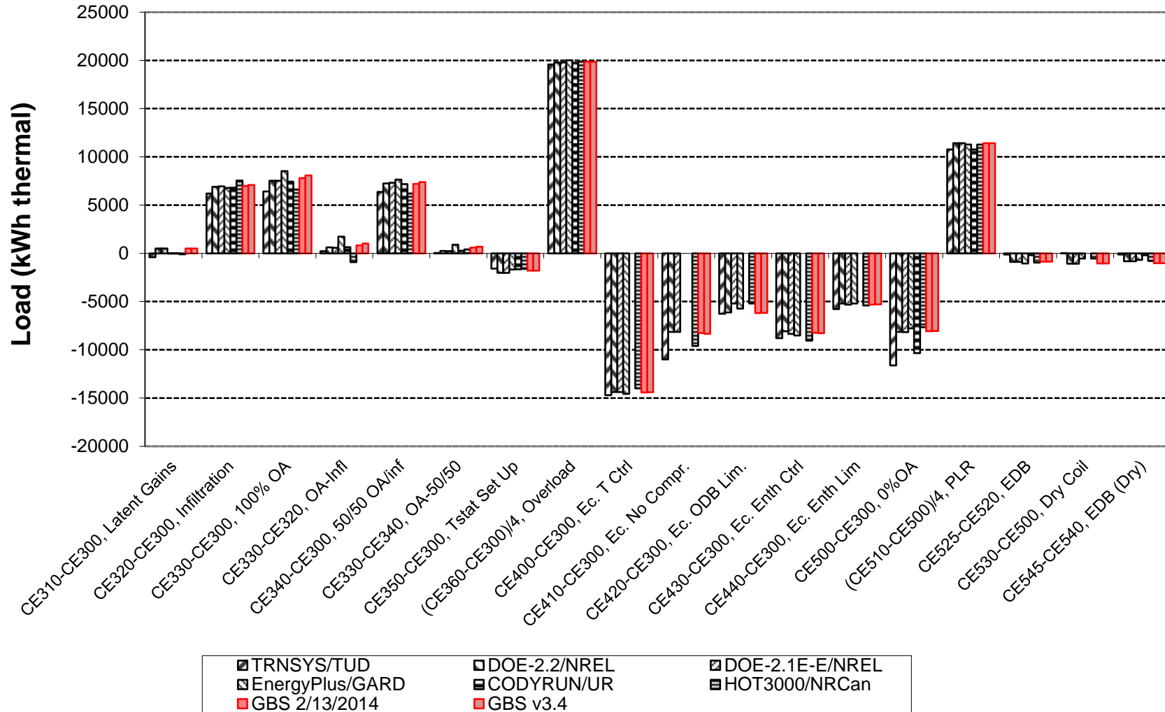
Figure B16.5.2-15. HVAC BESTEST: CE300 - CE545 Annual Sensible Cooling Load Sensitivities
